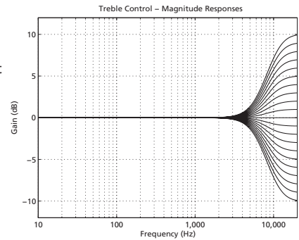
Figure 2: Frequency response measurements of all settings of the Treble control. Note that this response is applied to each input channel.
