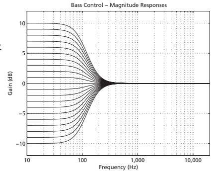
Figure 1: Frequency response measurements of all settings of the Bass control. Note that this response is applied to each input channel.
