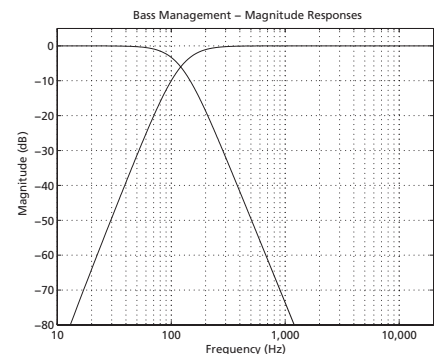
Figure 10: Magnitude response of the crossover used in the Bass Management system, showing an example with default frequency of 120 Hz.
