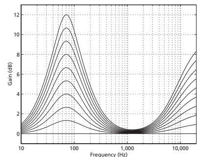
Figure 6: An example of the effect of the Loudness on the frequency response of the system at different volume settings. The lowest curve is for a high volume setting. The highest curve represents the response at a low volume setting. In this example, the Bass Max Boost is set to 12 dB and the Treble Max Boost is set to 9 dB.
