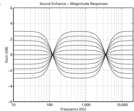
Figure 4: Frequency response measurements of all settings of the Sound Enhance control. Note that this response is applied to each input channel.
