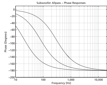
Figure 11: Phase response corresponding to three values for the Allpass Frequency setting, 20 Hz, 80 Hz, and 300 Hz.
