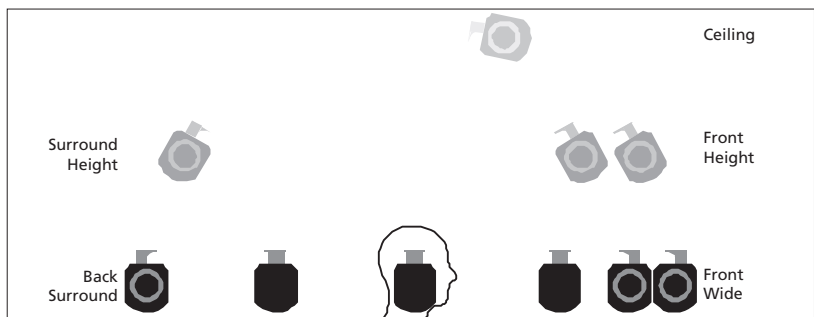
Figure 8: Side view of the loudspeaker positions associated with the speaker roles available in the television
