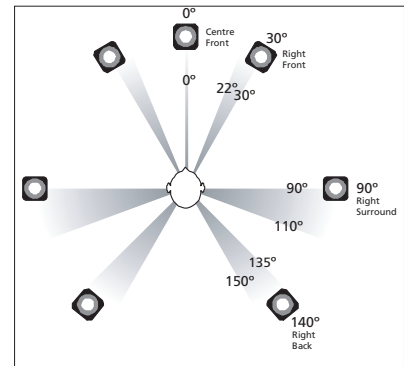
Figure 15: Recommended loudspeaker configuration for most 7.1 channel audio signals (provided that your television supports this setup). The grey zones show the commonly-accepted areas for surround and back loudspeaker placement. The actual placement of the loudspeakers (at 90 deg and 140 deg) shows the reference placement used at Bang & Olufsen for testing and tuning. Note that the placement of the subwoofer is better determined by your listening room's acoustics, but it is advisable to begin with a location near the centre front loudspeaker, if possible.
